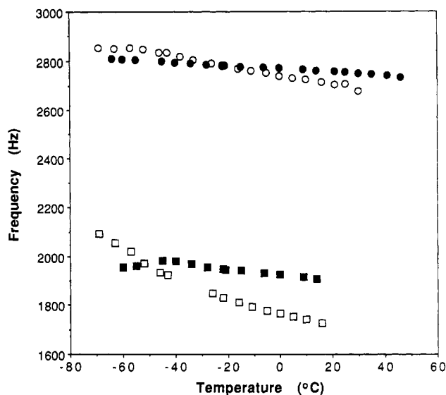
Figure 4. Plot of frequency versus temperature of the \text{H}_a (circles) and \text{H}_b (squares) resonances of C in 1:1 mixtures (hollow) and 1:2 mixtures (full) of C and G.
